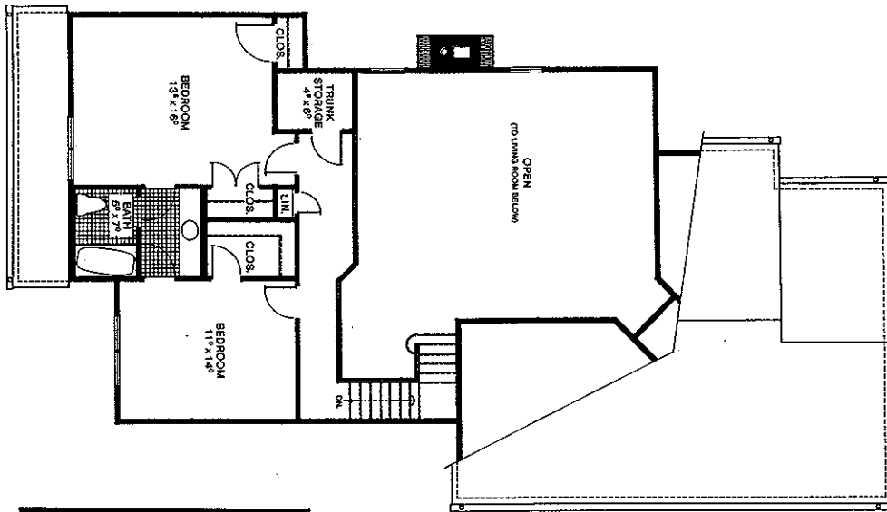
Second Floor
